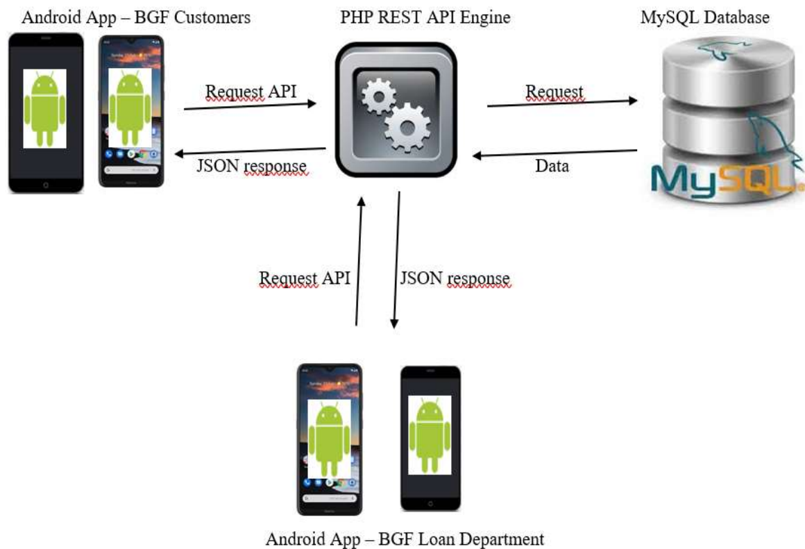
Figure 12: System architecture
