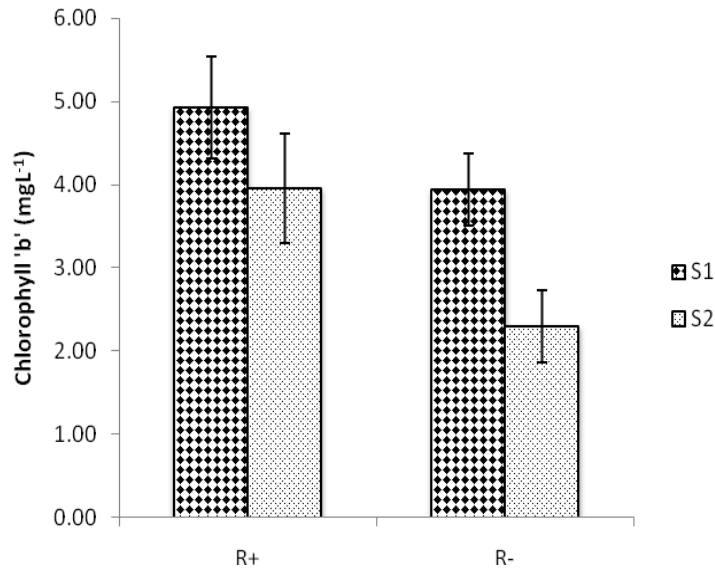
Figure 11: Interactive effects of Rhizobium and stress level on chlorophyll 'b' contents at vegetative stage in season (1) field experiment. +R: With Rhizobium , -R: Without Rhizobium . S1: Control, S2: Water stress at vegetative stage
