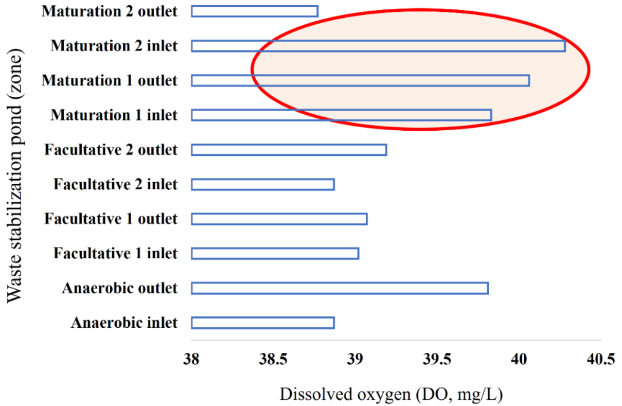
Figure 12. Levels of dissolved oxygen at different zones in the Arusha municipal WSPs. The encircled portion marks the maturation with high DO level.
